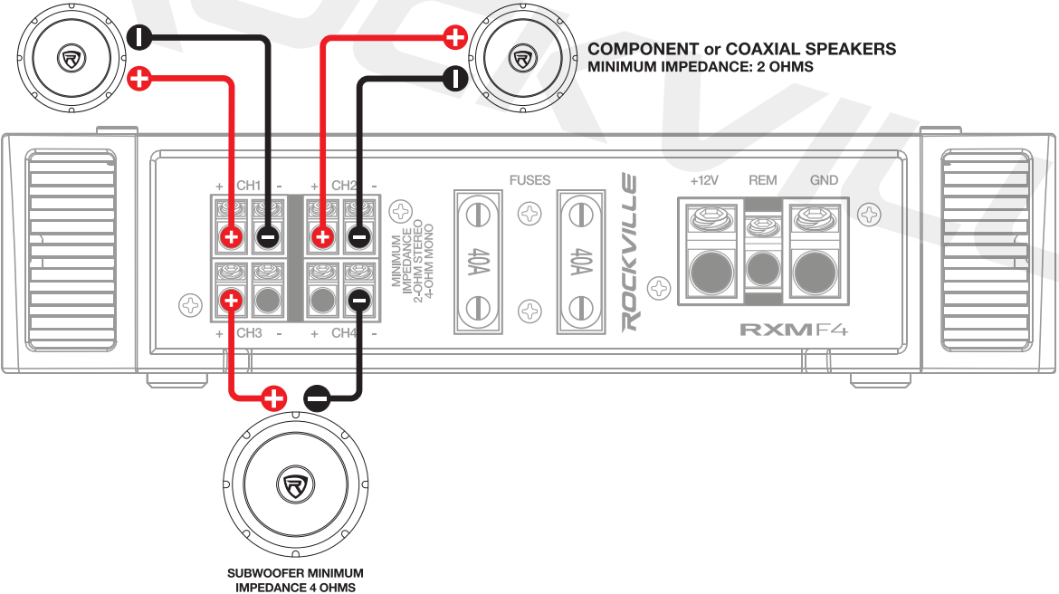
CHANNEL 3-4 CROSSOVER SWITCH SET TO LPF/BPF
