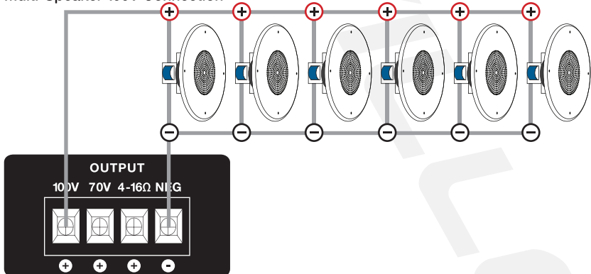
Multi-Speaker 100V Connection
