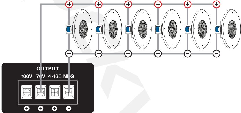
Multi-Speaker 70V Connection
