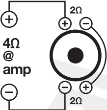
ONE 2Ω DVC WOOFER = 4Ω LOAD
