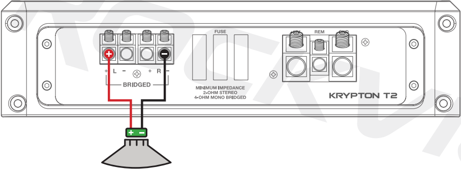
SUBWOOFER MINIMUM IMPEDANCE 4 OHMS
