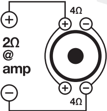
ONE 4Ω DVC WOOFER = 2Ω LOAD
