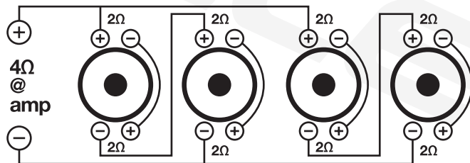
FOUR 2\Omega DVC WOOFERS = 4\Omega LOAD
