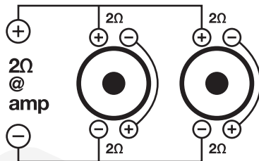
TWO 2\Omega DVC WOOFERS = 2\Omega LOAD
